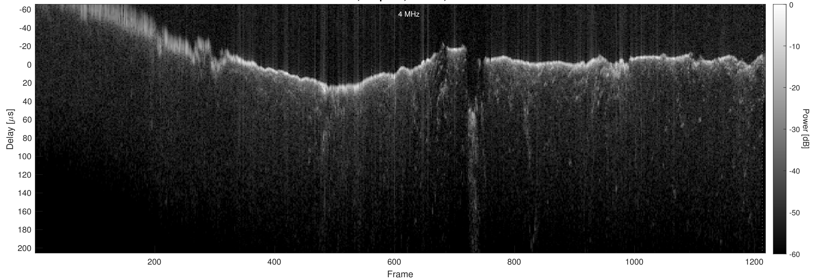
Orbit 19726, Chapman, Window, Channel 2
