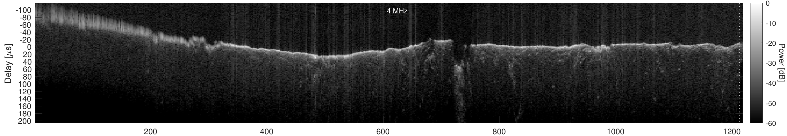
Orbit 19726, Window, Channel 2, Optimized
