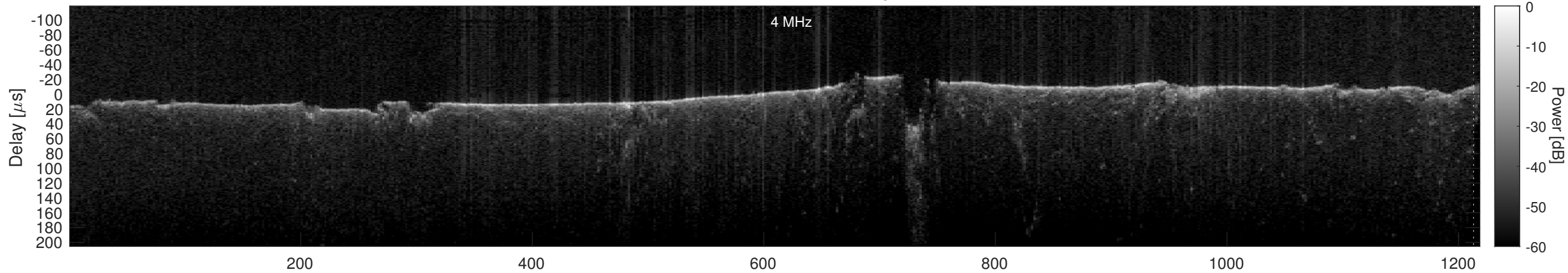
Orbit 19726, Cluttergram
