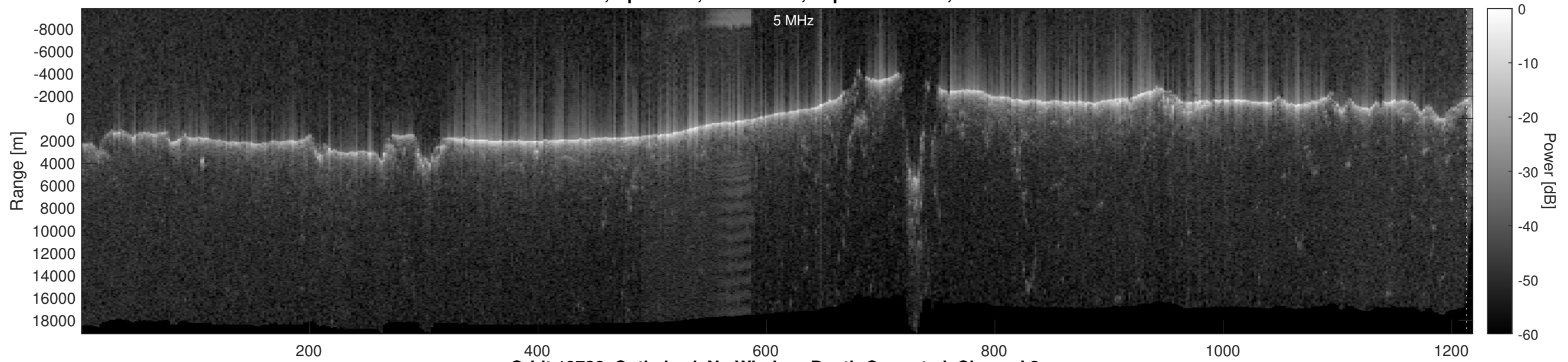
Orbit 19726, Optimized, No Window, Depth-Corrected, Channel 2
