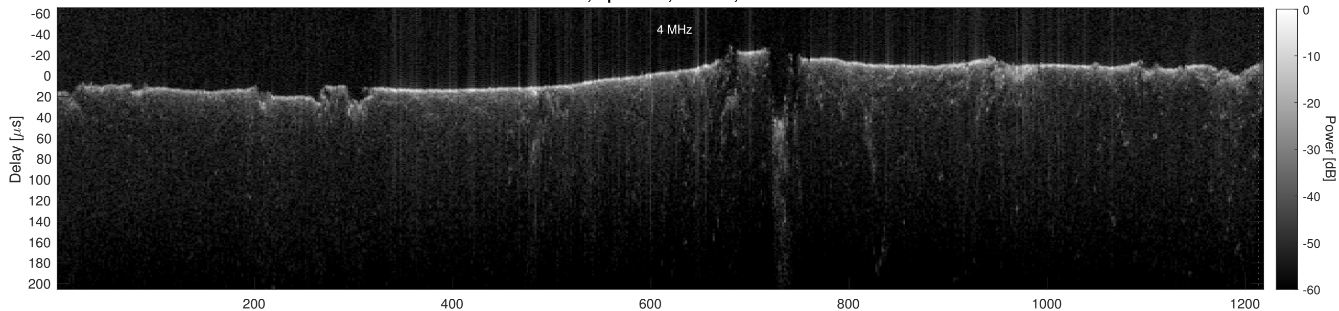
Orbit 19726, Cluttergram
