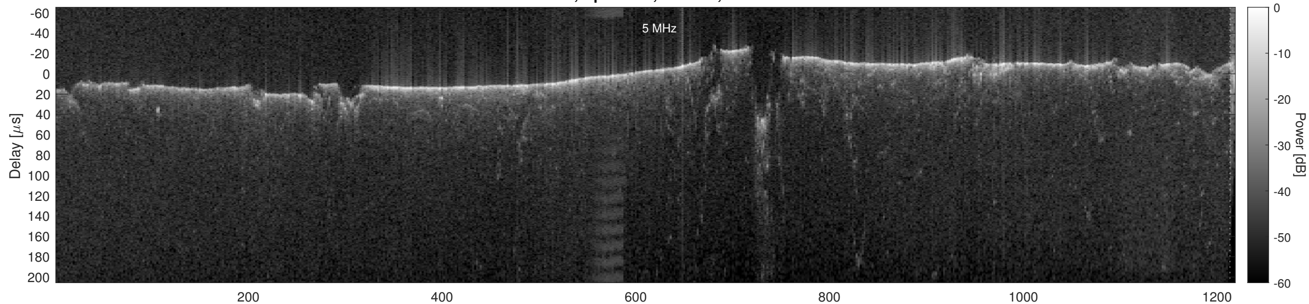
Orbit 19726, Optimized, Window, Channel 2
