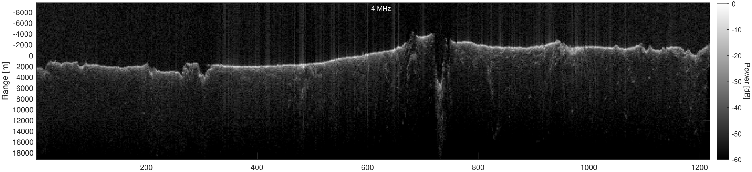
Orbit 19726, Depth-Corrected Cluttergram
