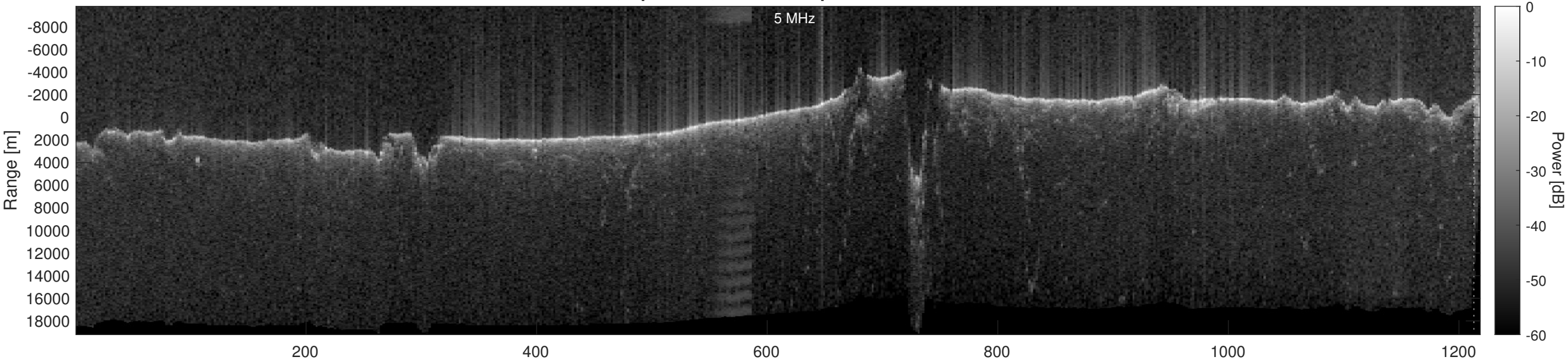
Orbit 19726, Optimized, Window, Depth-Corrected, Channel 2
