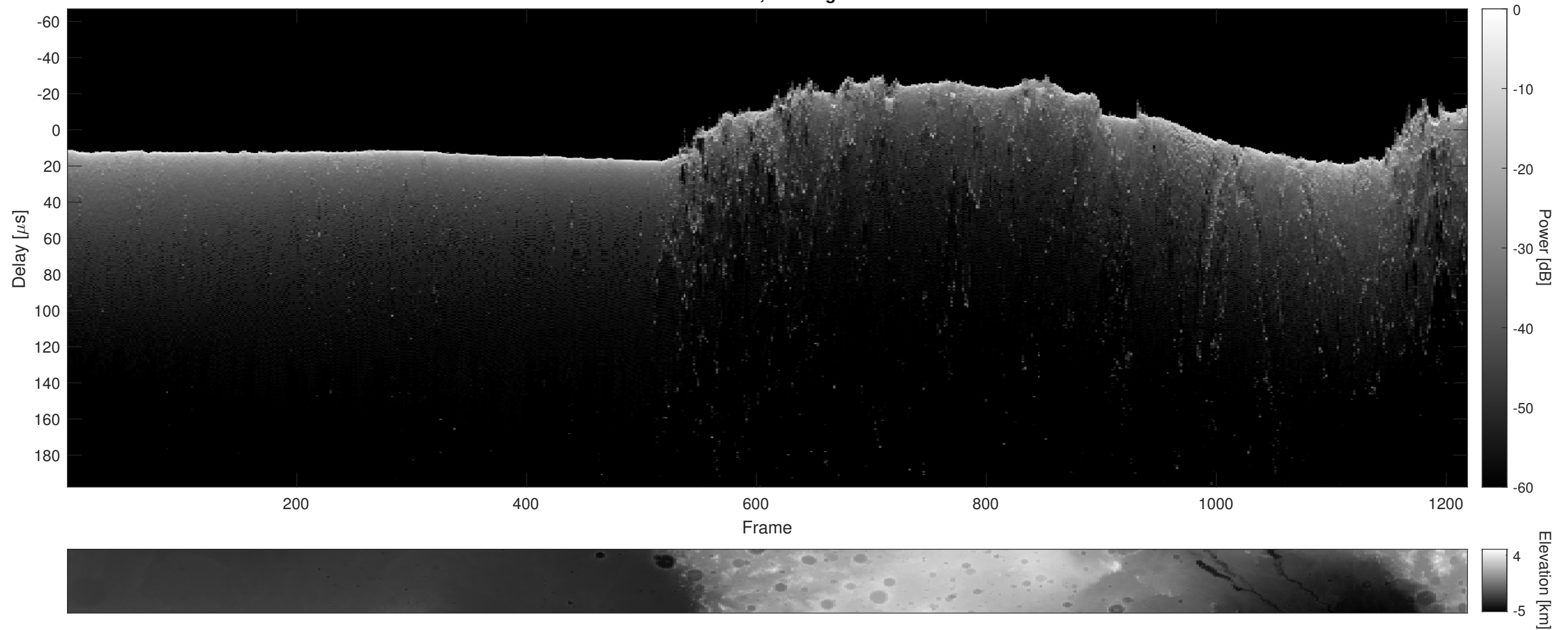
Orbit 19728, Cluttergram
