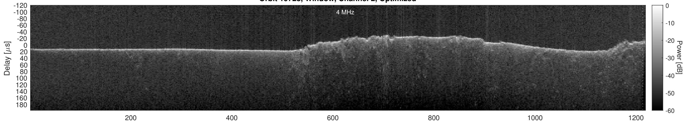
Orbit 19728, Cluttergram
