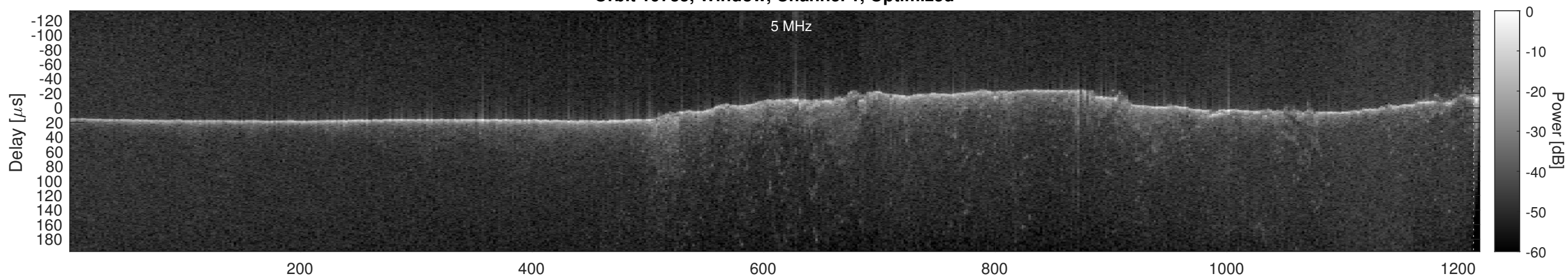
Orbit 19735, Cluttergram
