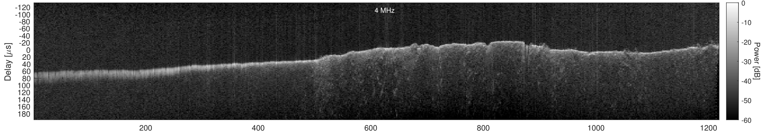
Orbit 19735, Window, Channel 2, Chapman
