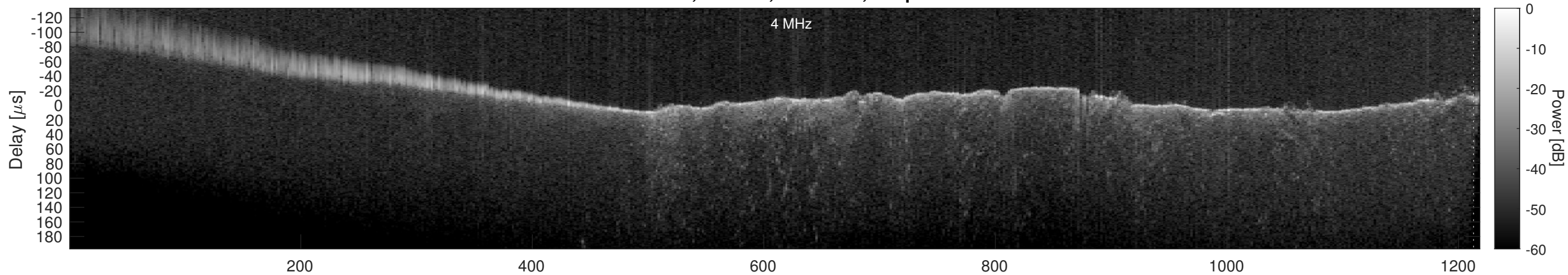
Orbit 19735, Window, Channel 2, Optimized
