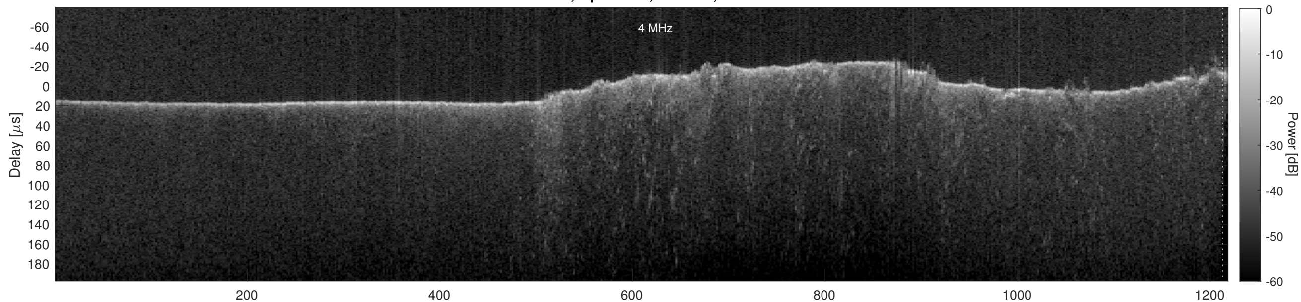
Orbit 19735, Cluttergram
