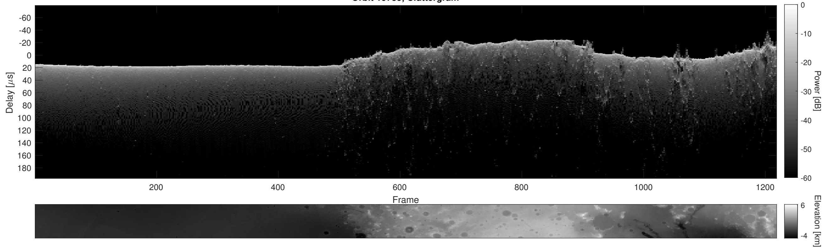
Orbit 19735, Cluttergram
