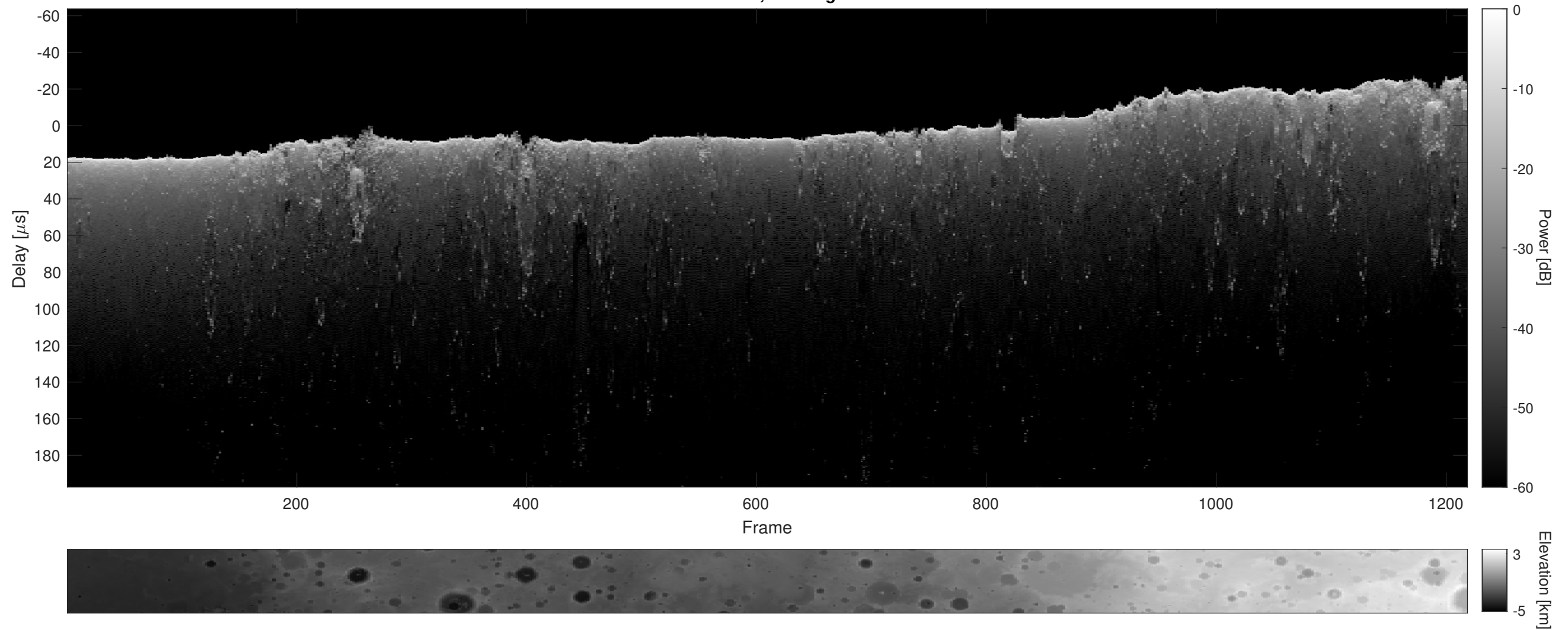
Orbit 19736, Cluttergram
