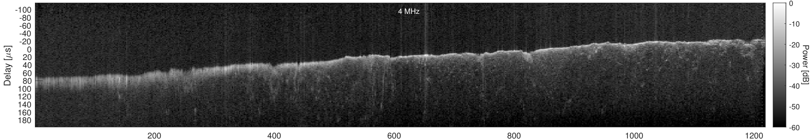
Orbit 19736, Window, Channel 2, Chapman
