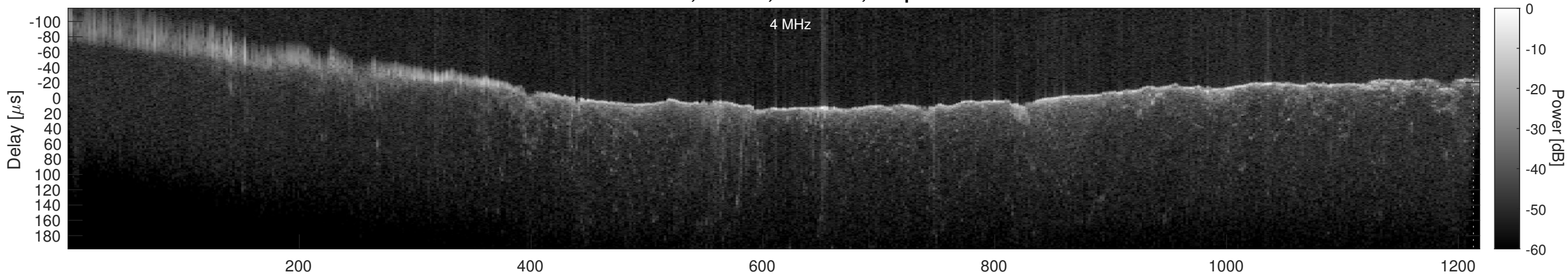
Orbit 19736, Window, Channel 2, Optimized
