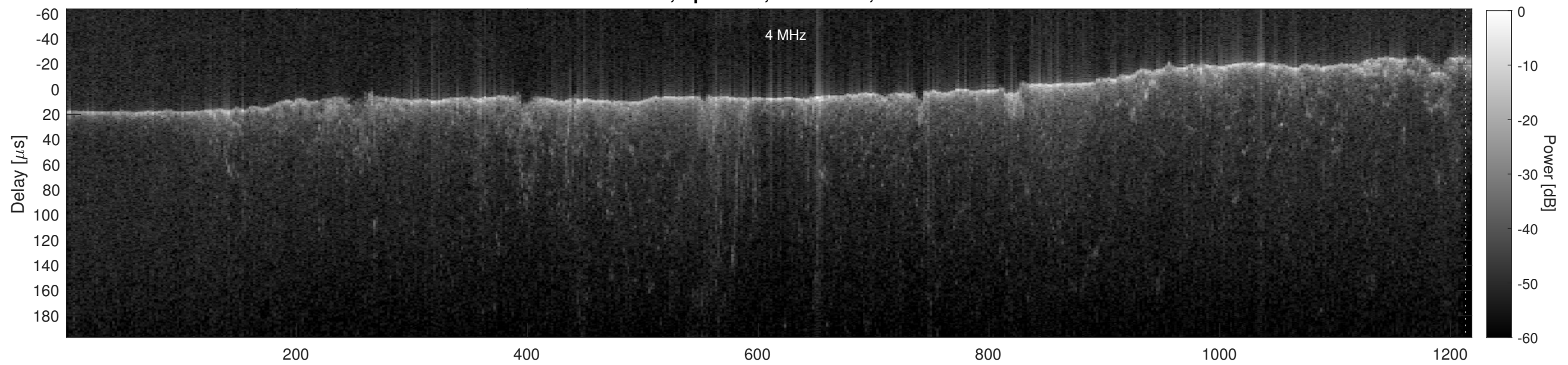
Orbit 19736, Cluttergram
