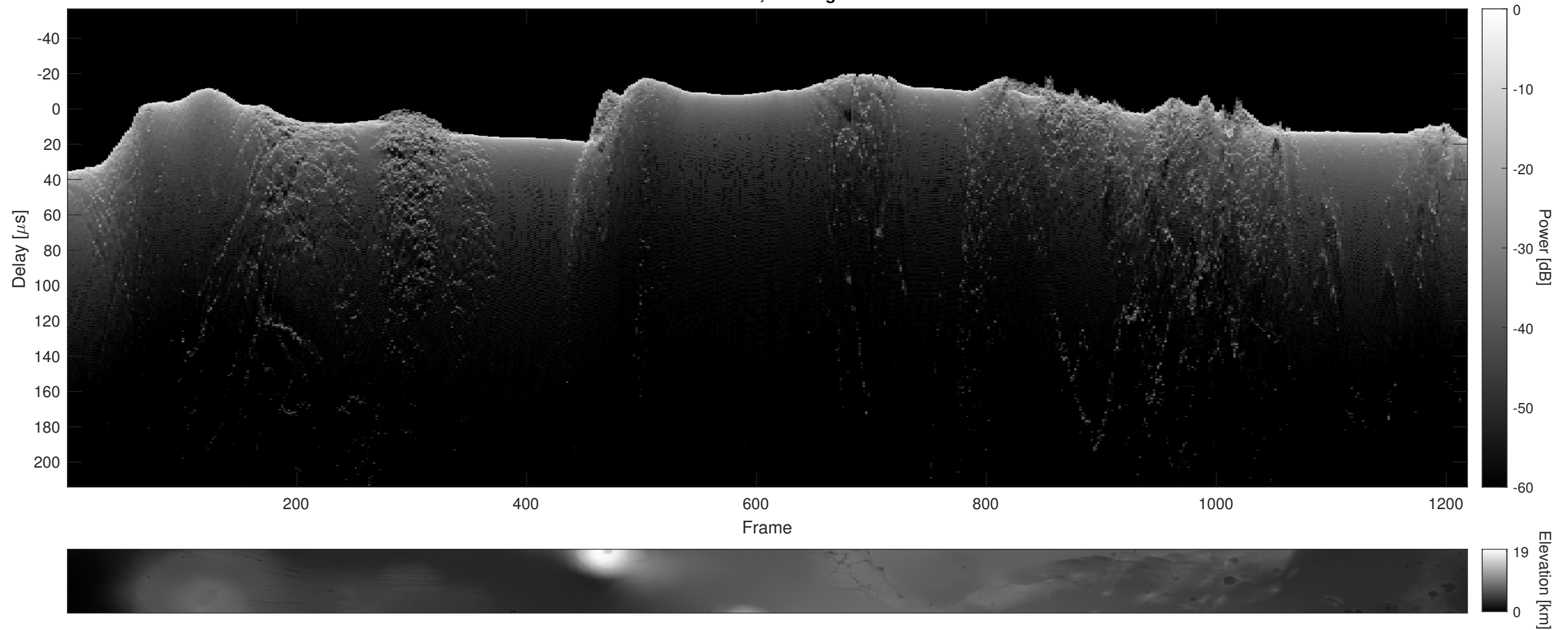
Orbit 19737, Cluttergram
