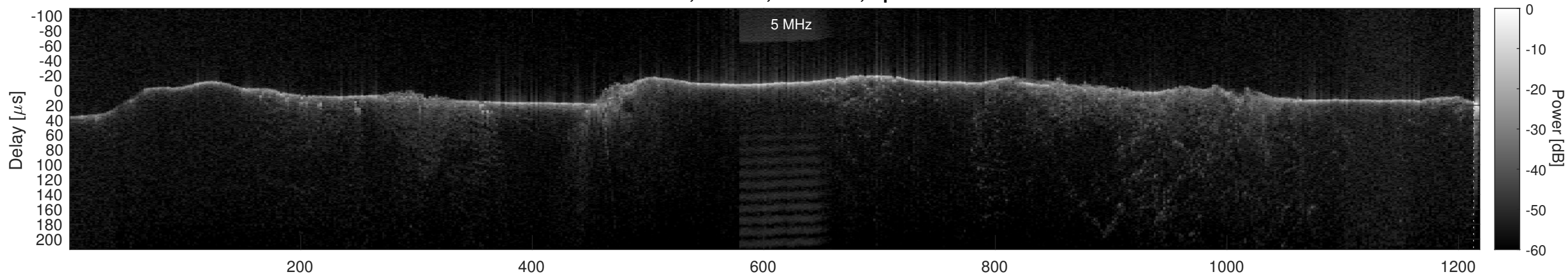
Orbit 19737, Cluttergram
