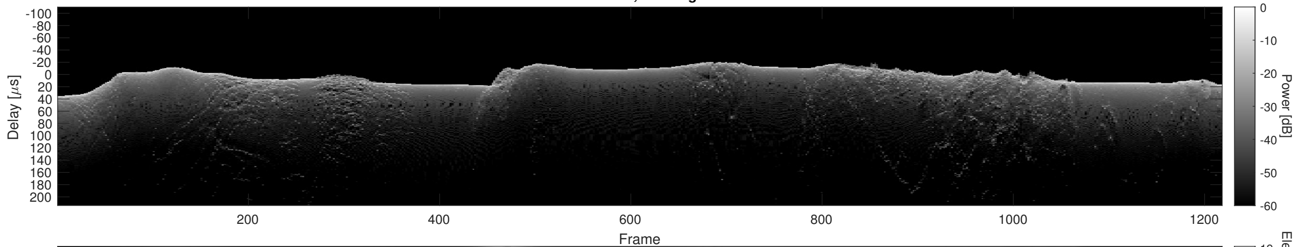
Orbit 19737, Cluttergram
