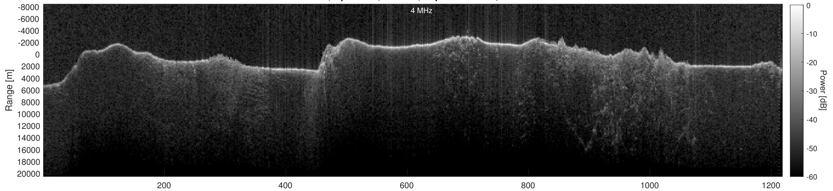
Orbit 19737, Depth-Corrected Cluttergram
