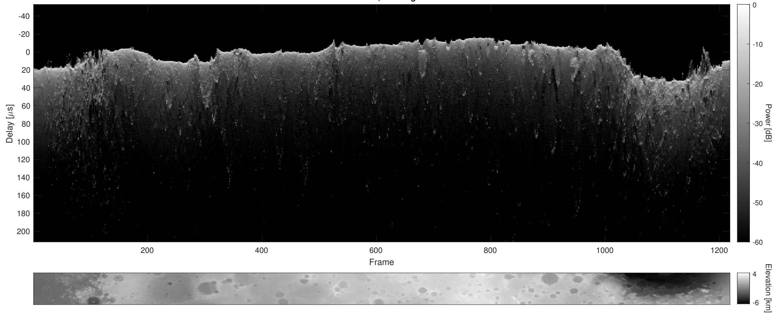
Orbit 19739, Cluttergram
