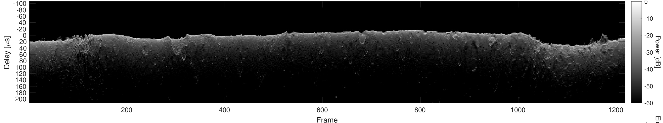
Orbit 19739, Cluttergram
