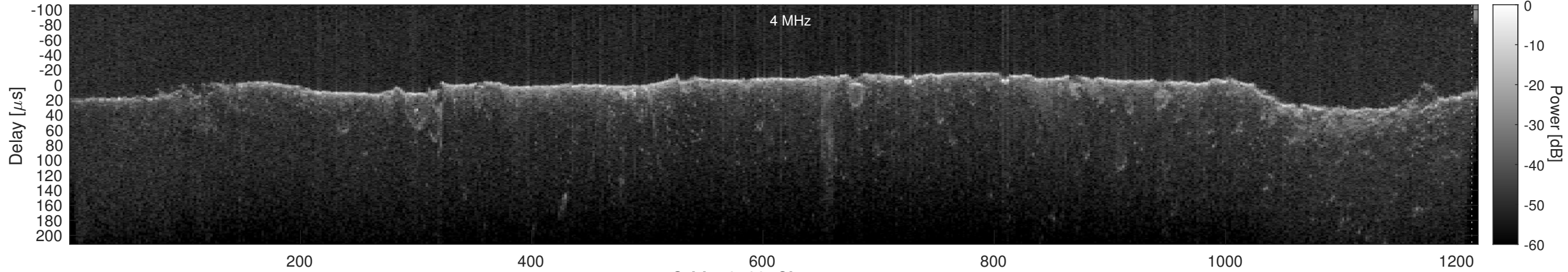
Orbit 19739, Cluttergram
