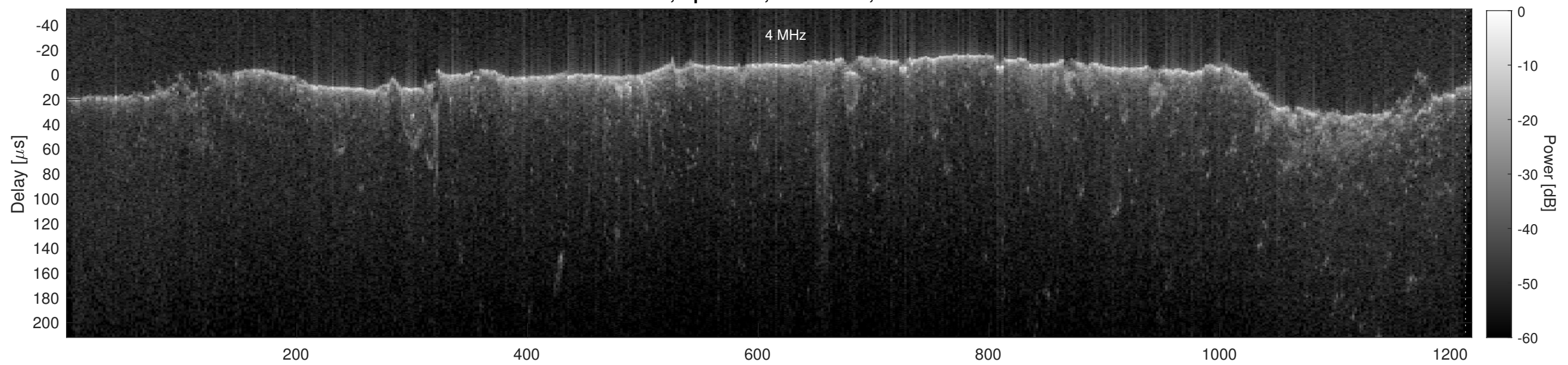
Orbit 19739, Cluttergram
