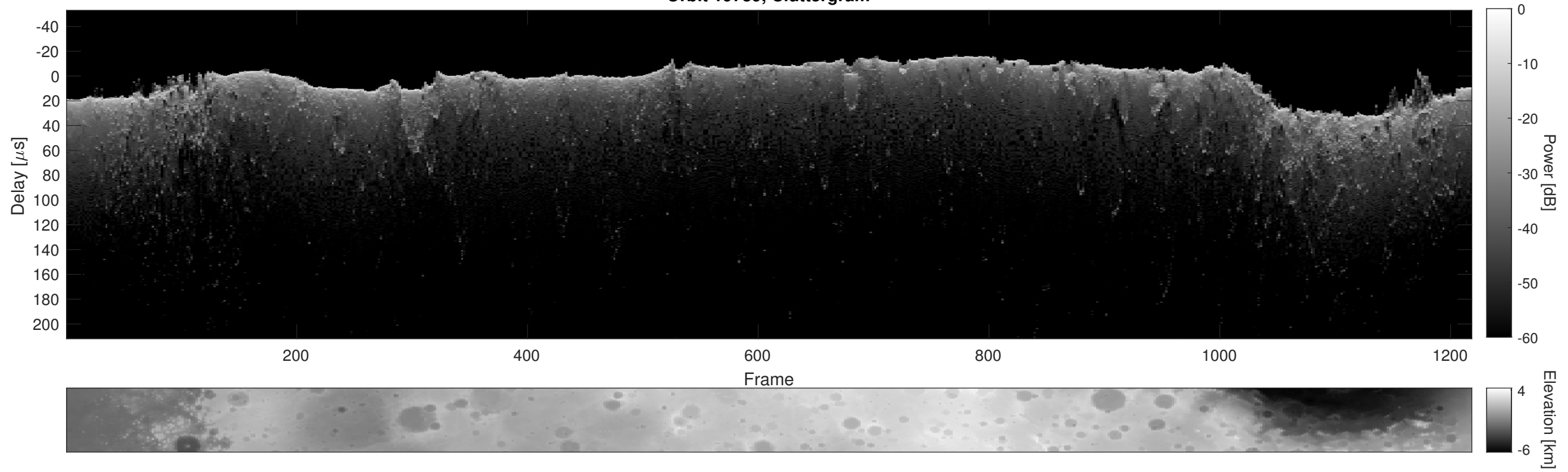
Orbit 19739, Cluttergram
