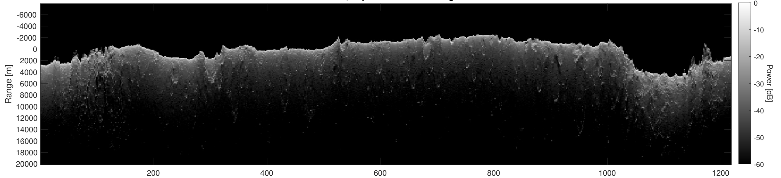
Orbit 19739, Depth-Corrected Cluttergram
