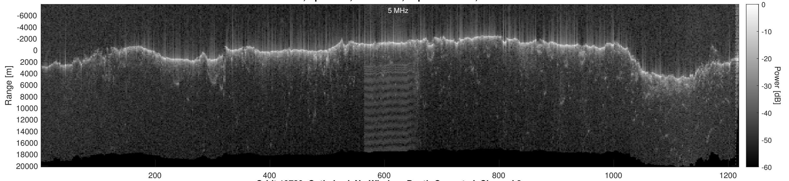
Orbit 19739, Optimized, No Window, Depth-Corrected, Channel 2
