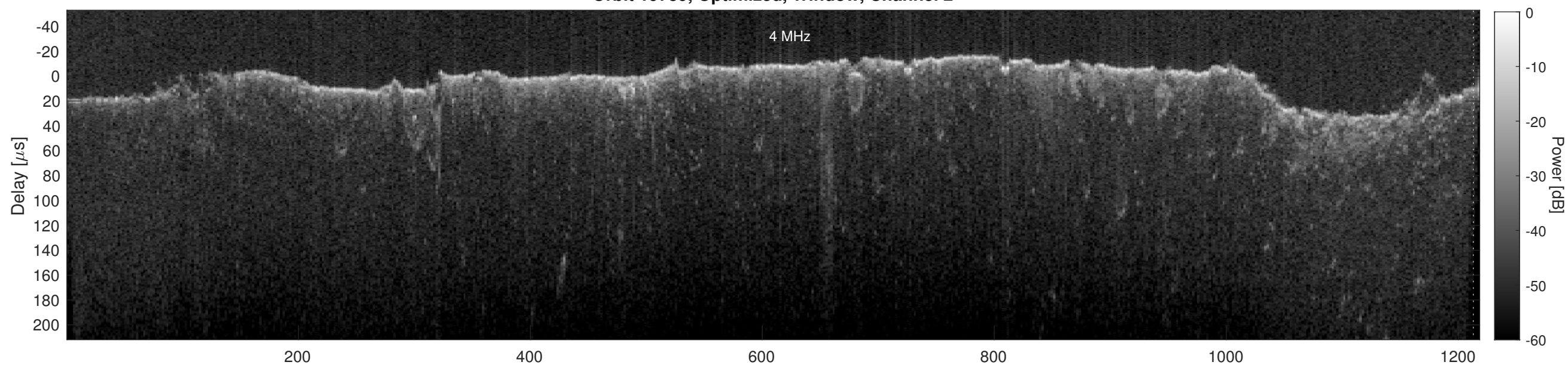
Orbit 19739, Cluttergram
