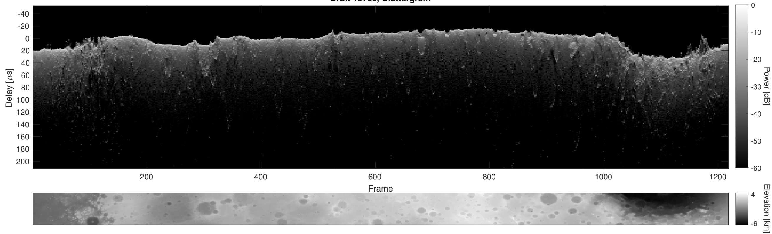
Orbit 19739, Cluttergram
