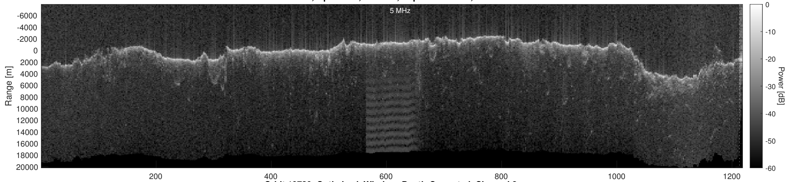
Orbit 19739, Optimized, Window, Depth-Corrected, Channel 2
