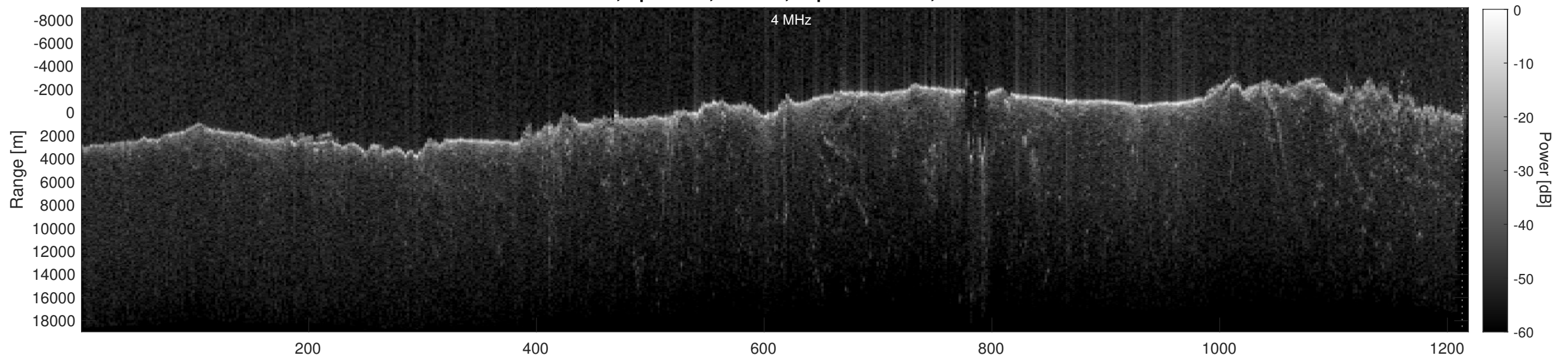
Orbit 19740, Depth-Corrected Cluttergram
