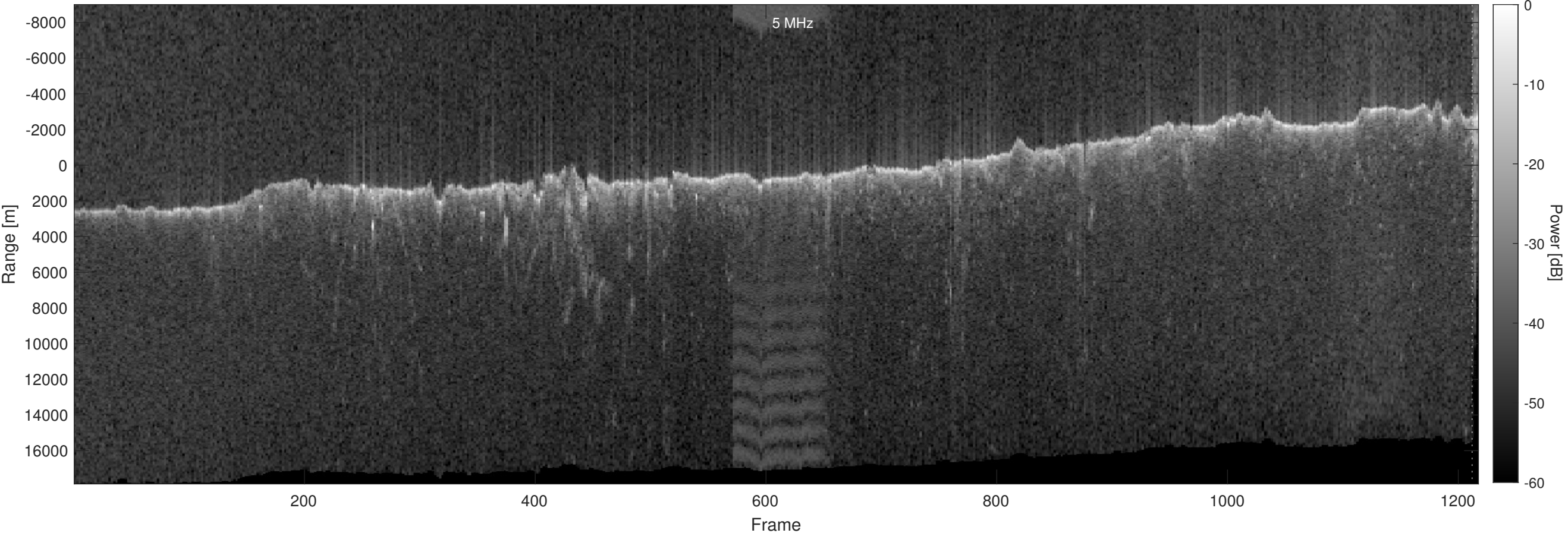
Orbit 19750, Optimized, Window, Depth-Corrected, Channel 2
