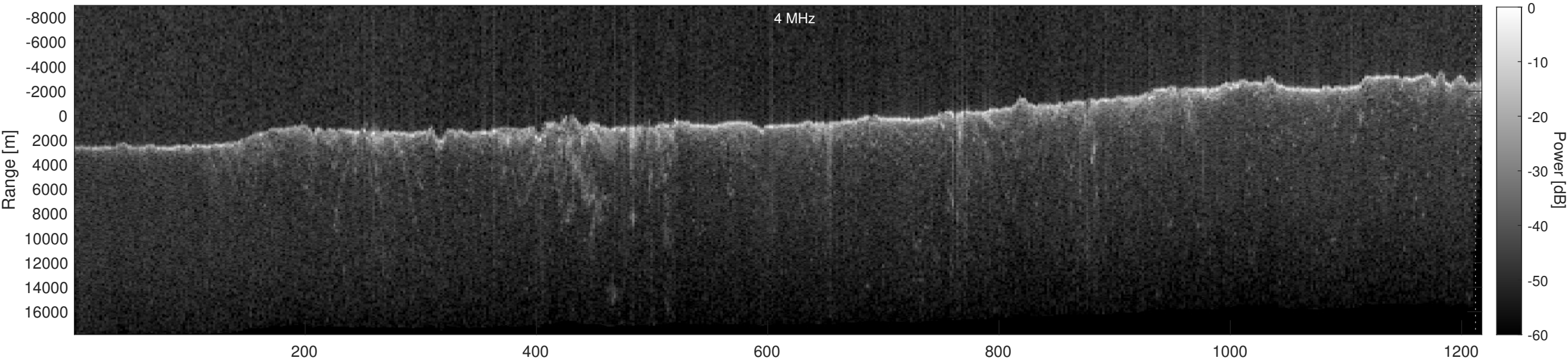
Orbit 19750, Depth-Corrected Cluttergram
