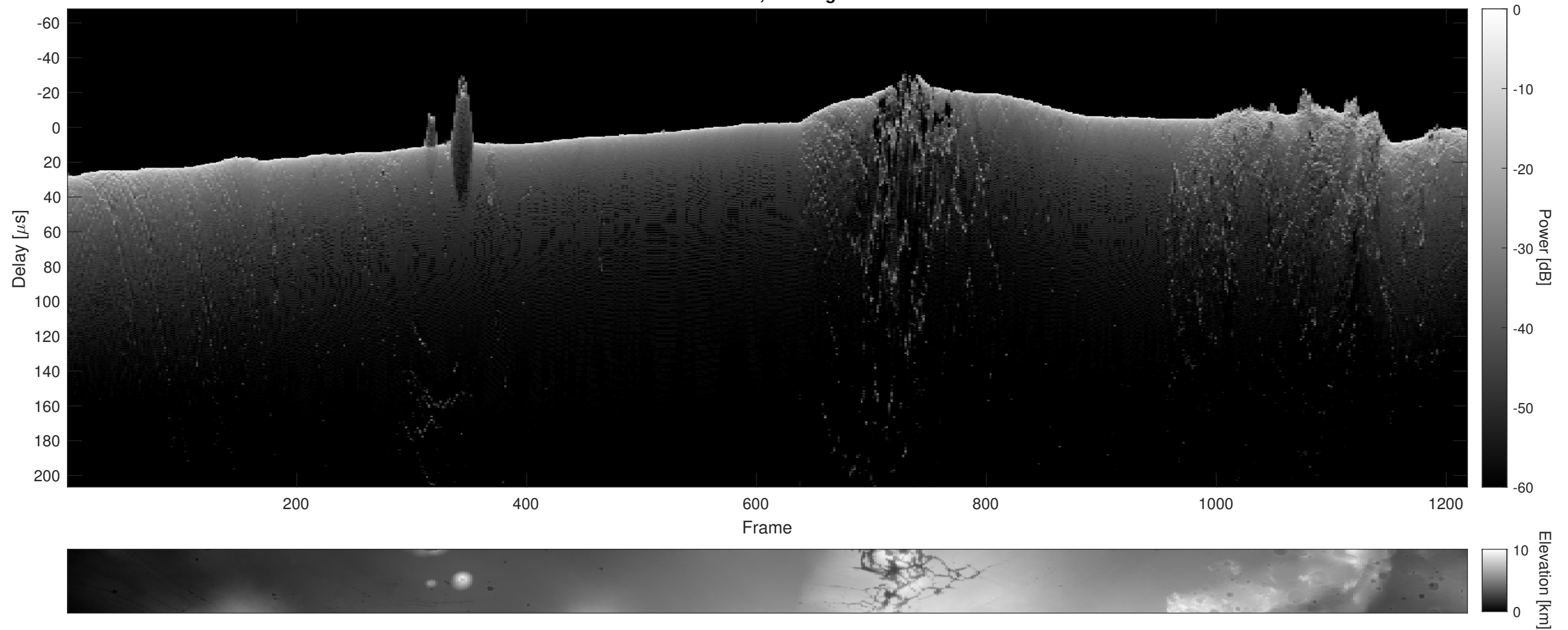
Orbit 19751, Cluttergram
