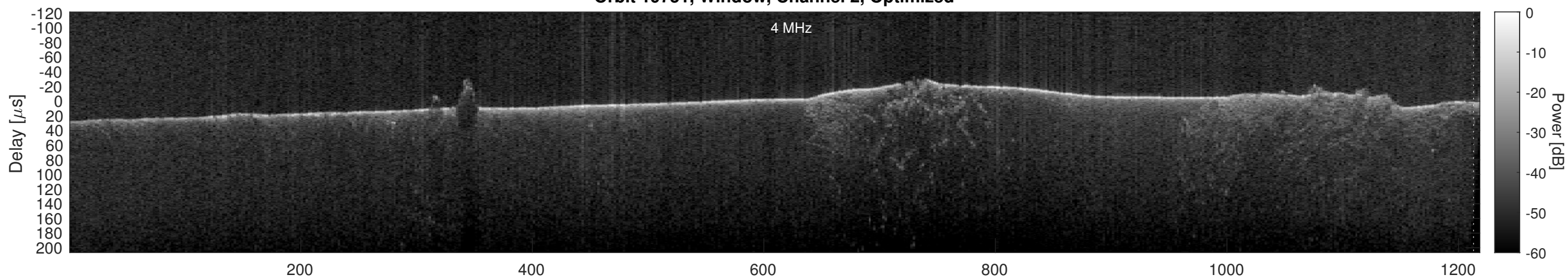
Orbit 19751, Cluttergram
