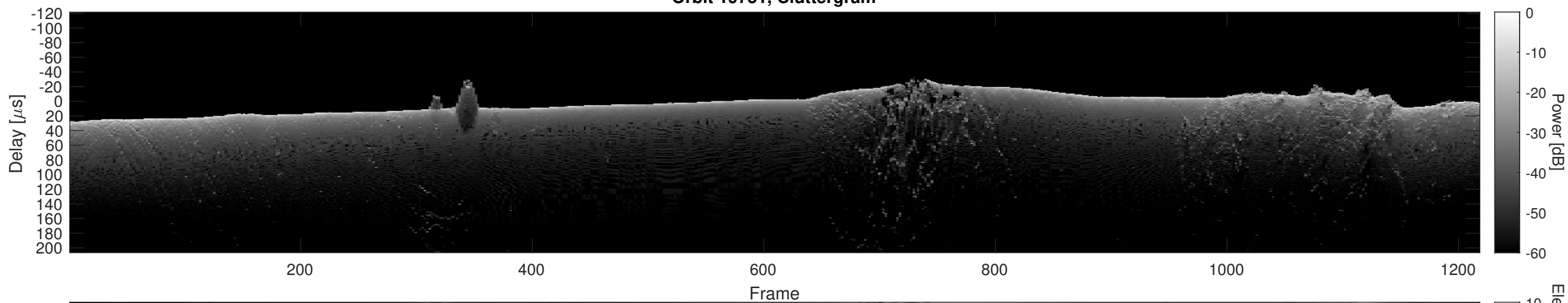
Orbit 19751, Cluttergram
