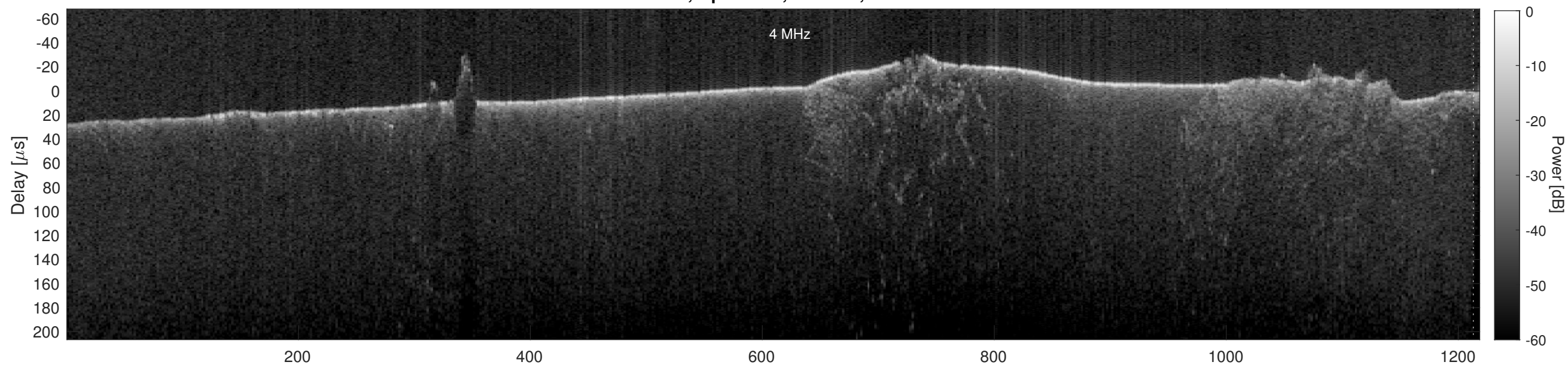
Orbit 19751, Cluttergram
