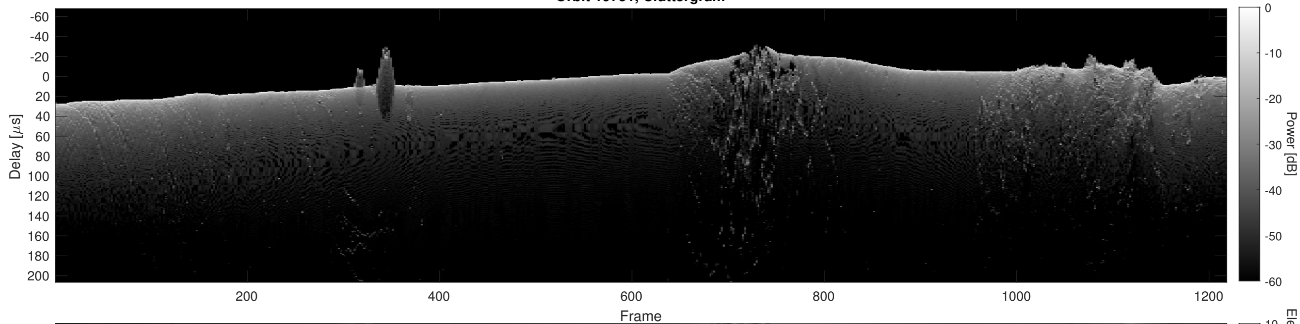
Orbit 19751, Cluttergram
