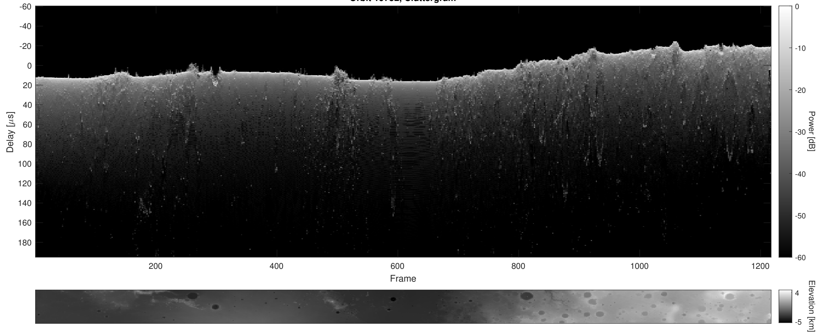
Orbit 19752, Cluttergram
