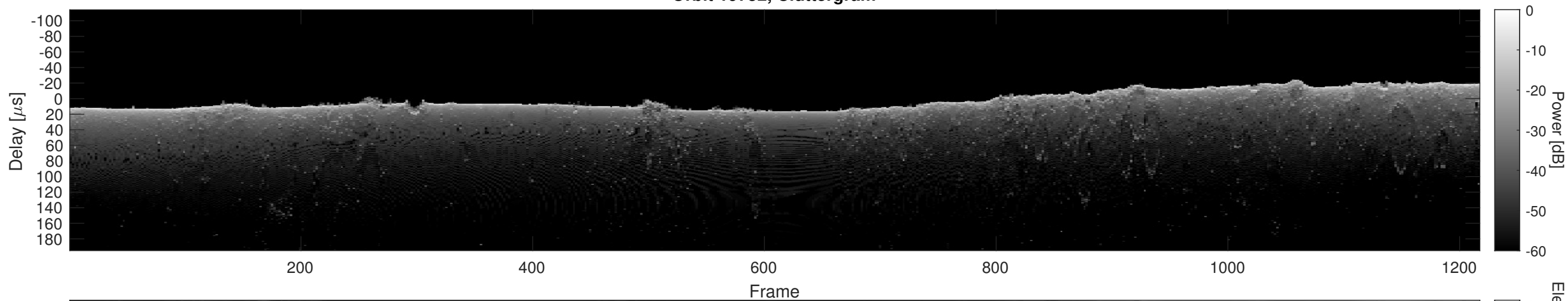
Orbit 19752, Cluttergram
