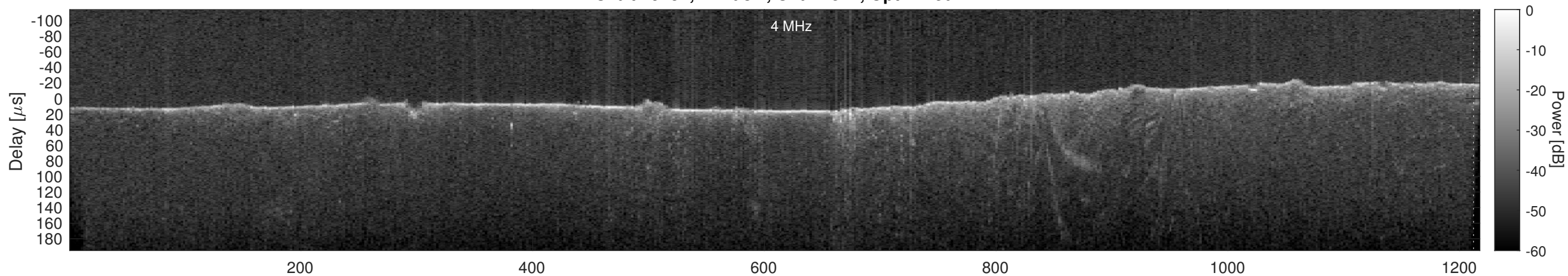
Orbit 19752, Cluttergram
