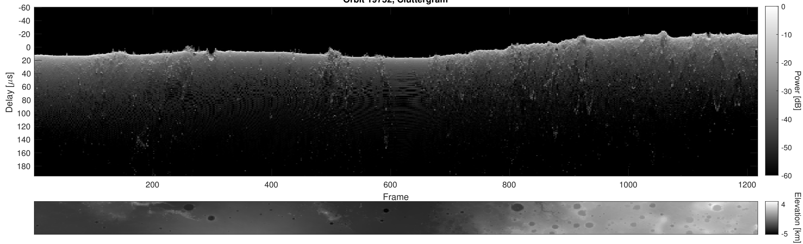
Orbit 19752, Cluttergram
