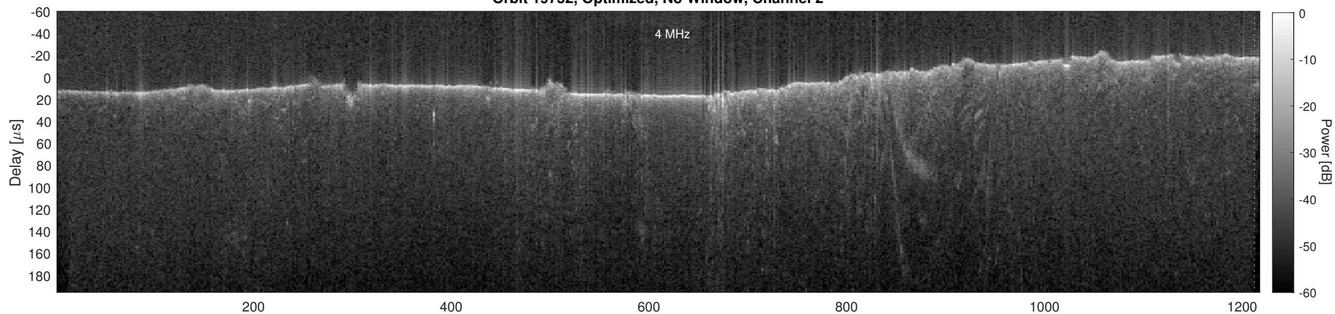
Orbit 19752, Cluttergram
