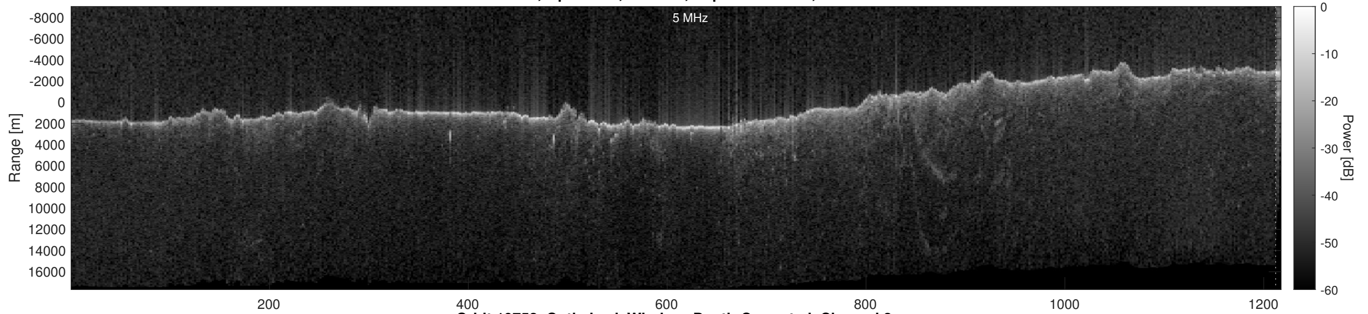
Orbit 19752, Optimized, Window, Depth-Corrected, Channel 2
