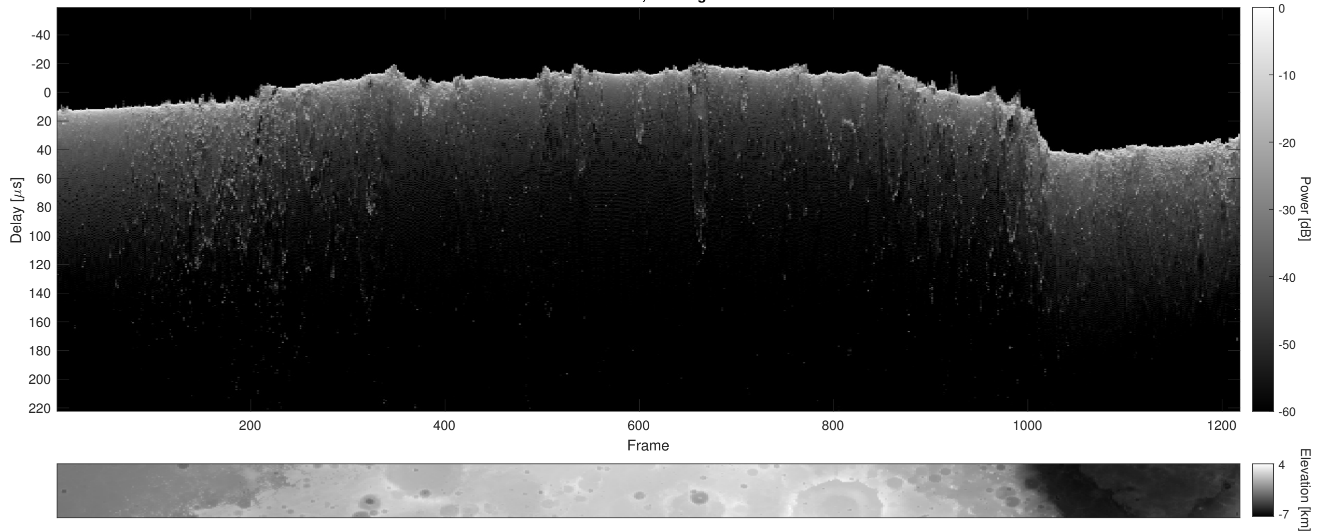
Orbit 19753, Cluttergram
