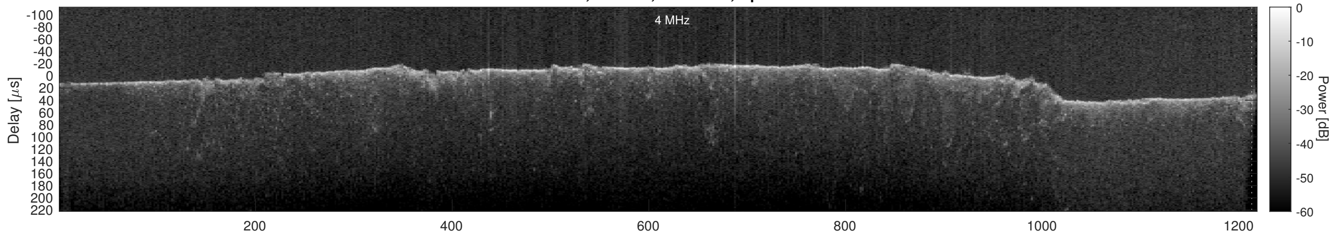
Orbit 19753, Cluttergram
