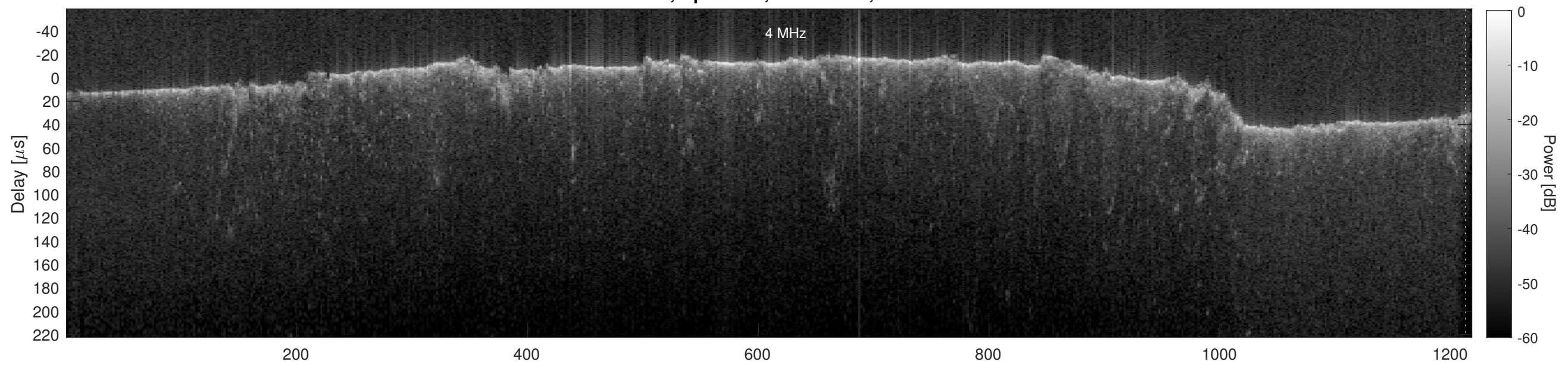
Orbit 19753, Cluttergram
