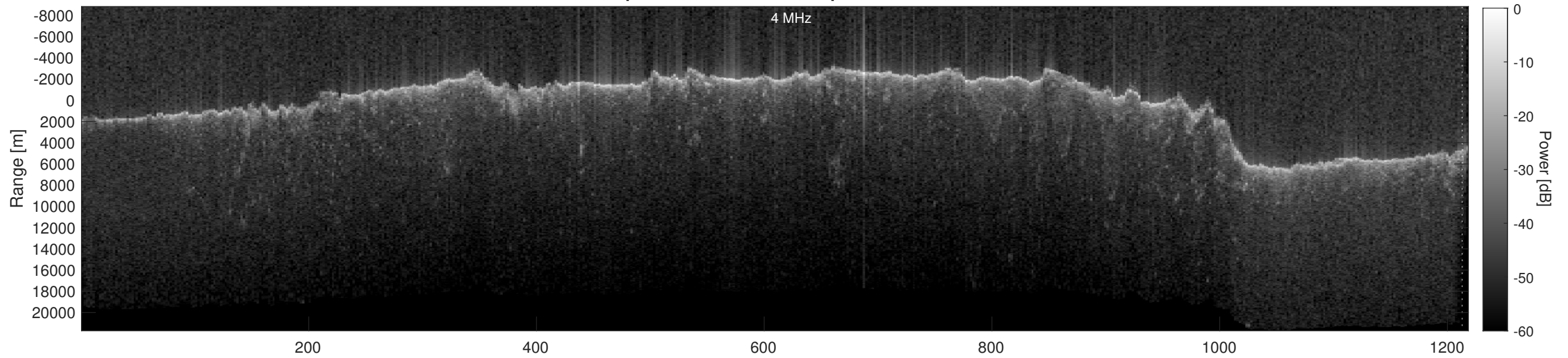
Orbit 19753, Depth-Corrected Cluttergram
