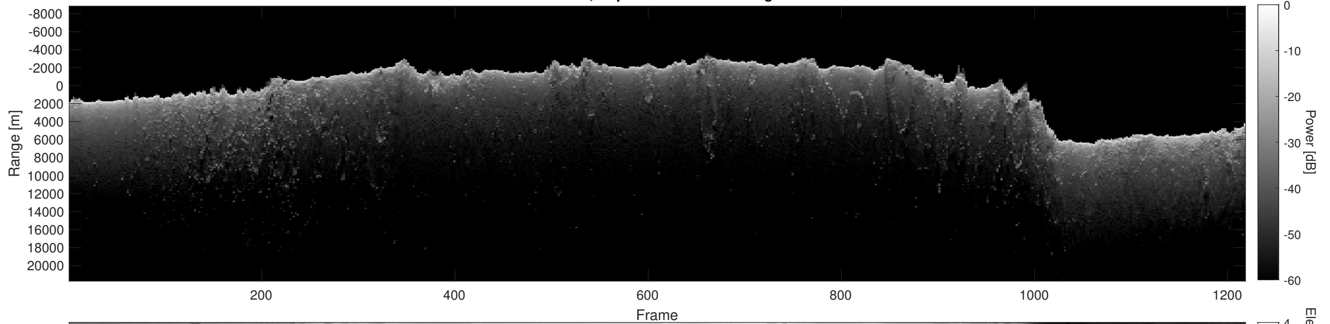
Orbit 19753, Depth-Corrected Cluttergram
