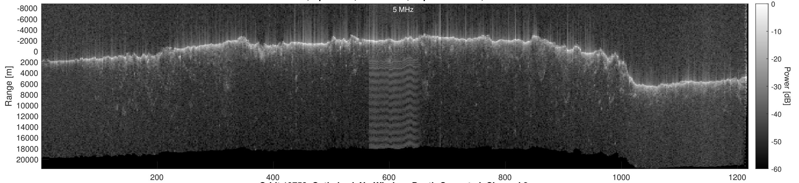
Orbit 19753, Optimized, No Window, Depth-Corrected, Channel 2
