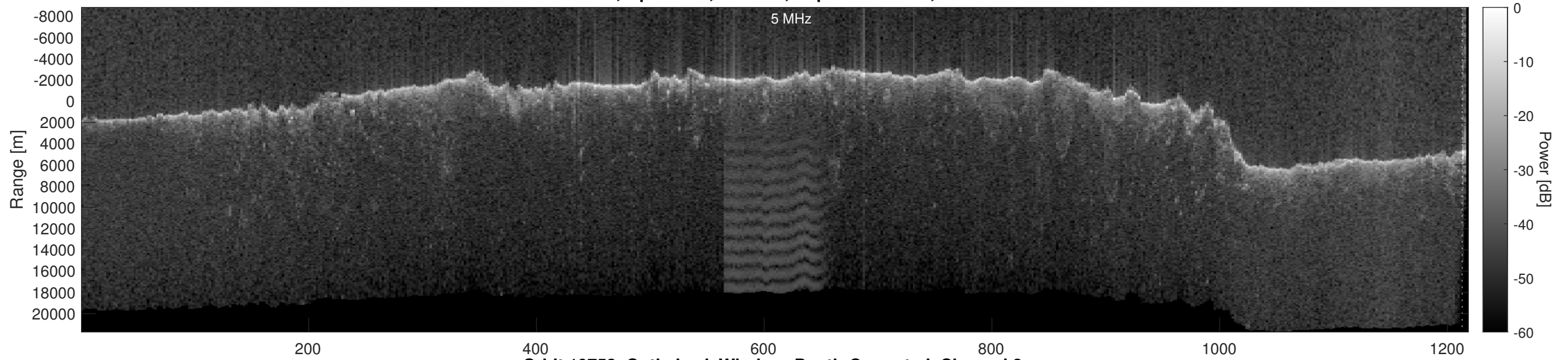
Orbit 19753, Optimized, Window, Depth-Corrected, Channel 2
