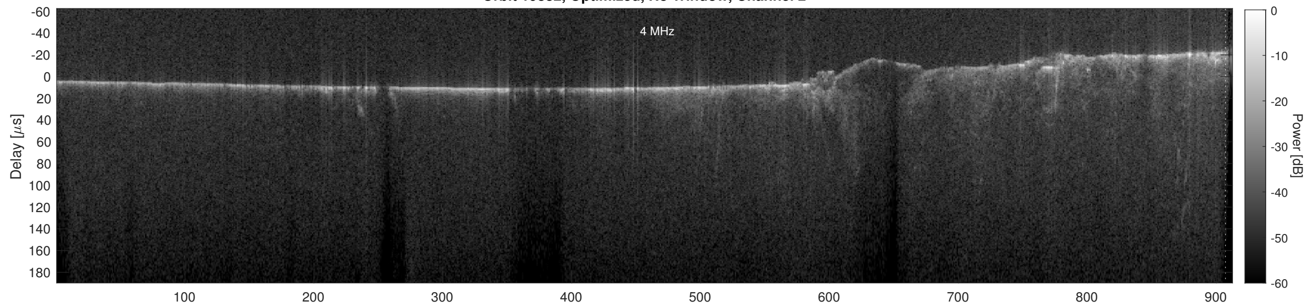
Orbit 19882, Cluttergram
