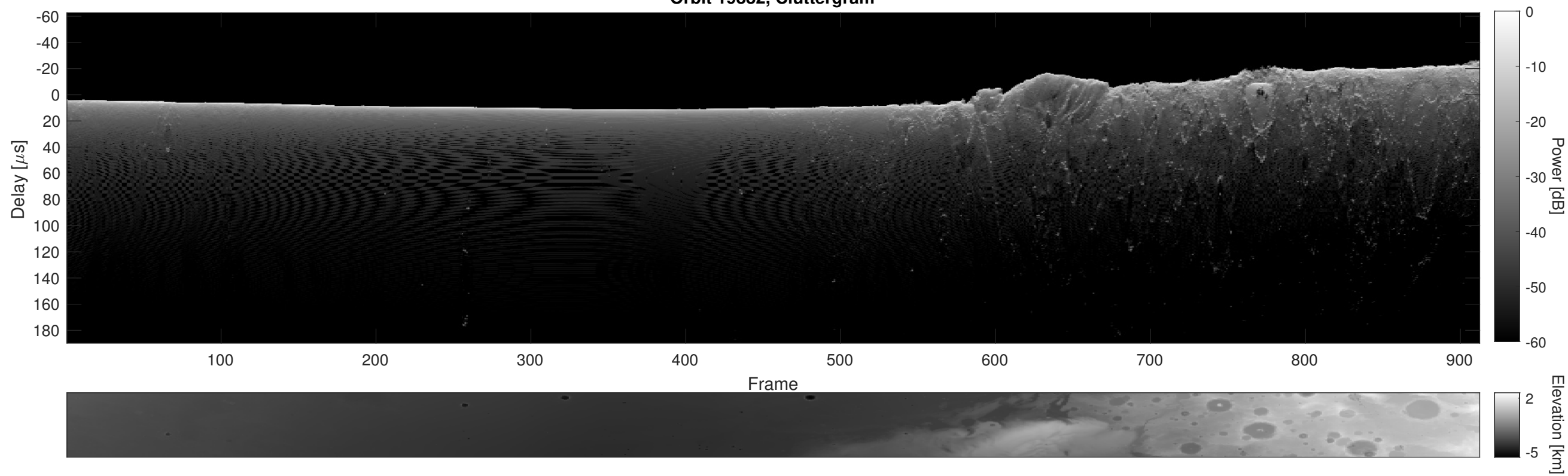
Orbit 19882, Cluttergram
