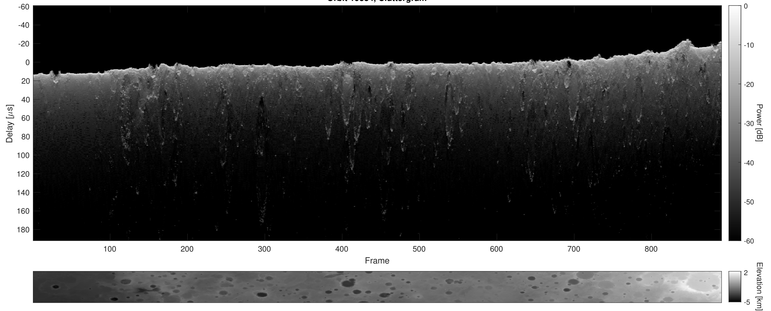
Orbit 19884, Cluttergram
