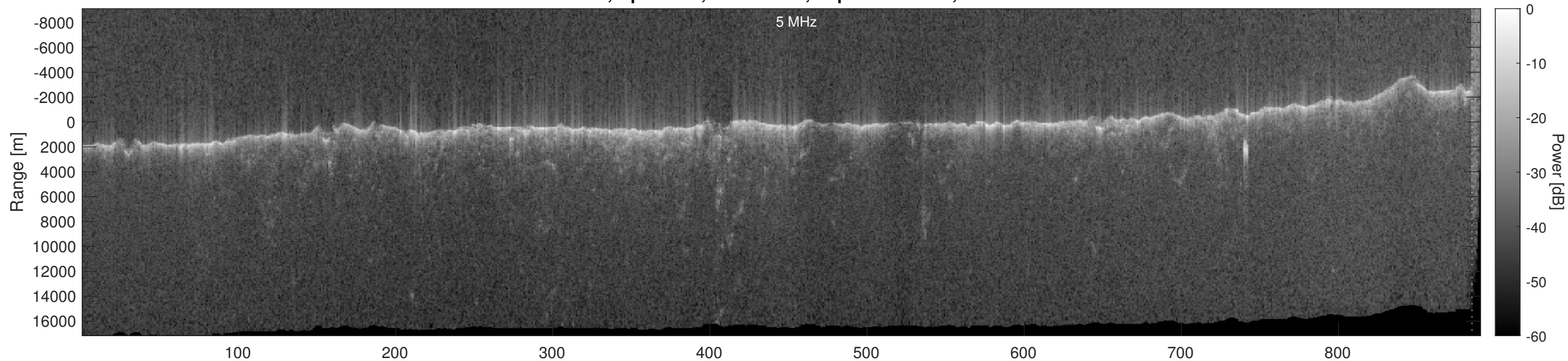
Orbit 19884, Optimized, No Window, Depth-Corrected, Channel 2
