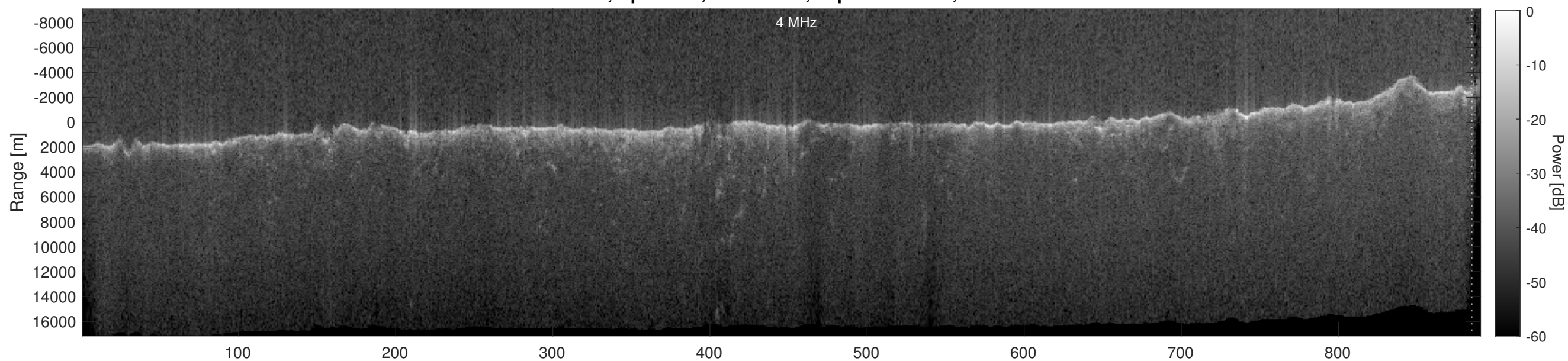
Orbit 19884, Depth-Corrected Cluttergram
