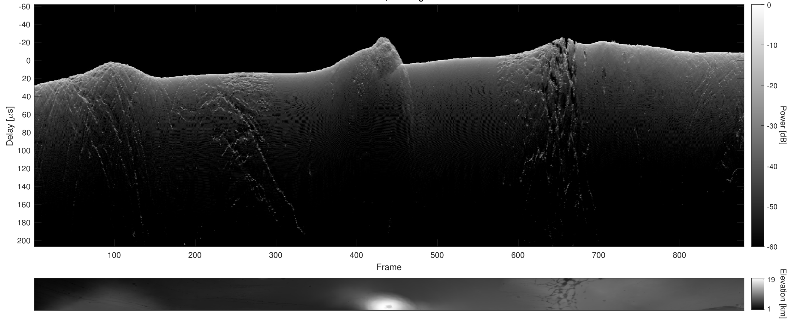
Orbit 19885, Cluttergram
