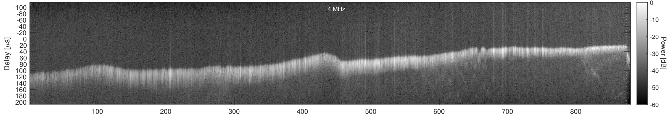
Orbit 19885, Window, Channel 2, Chapman
