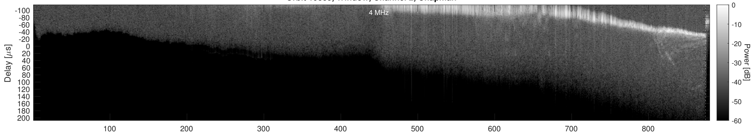
Orbit 19885, Window, Channel 2, Optimized
