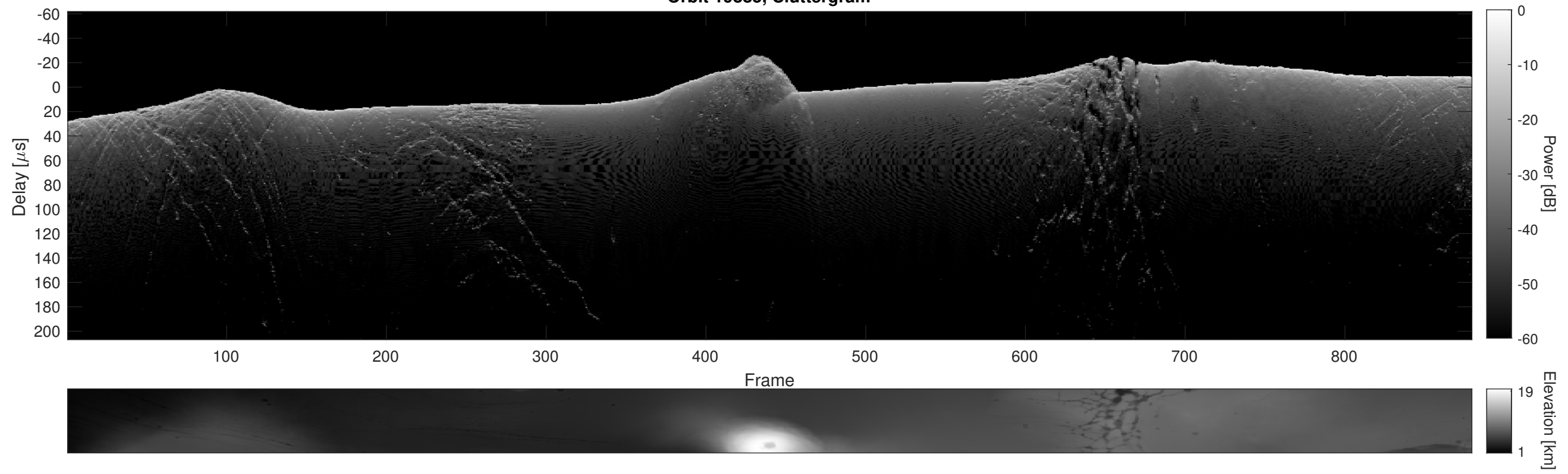
Orbit 19885, Cluttergram
