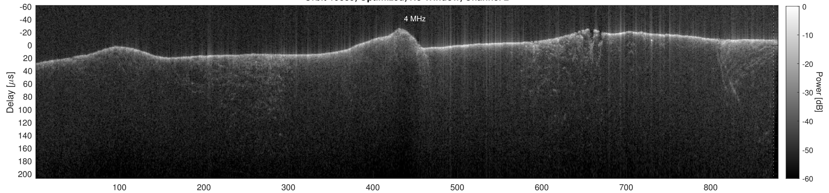
Orbit 19885, Cluttergram
