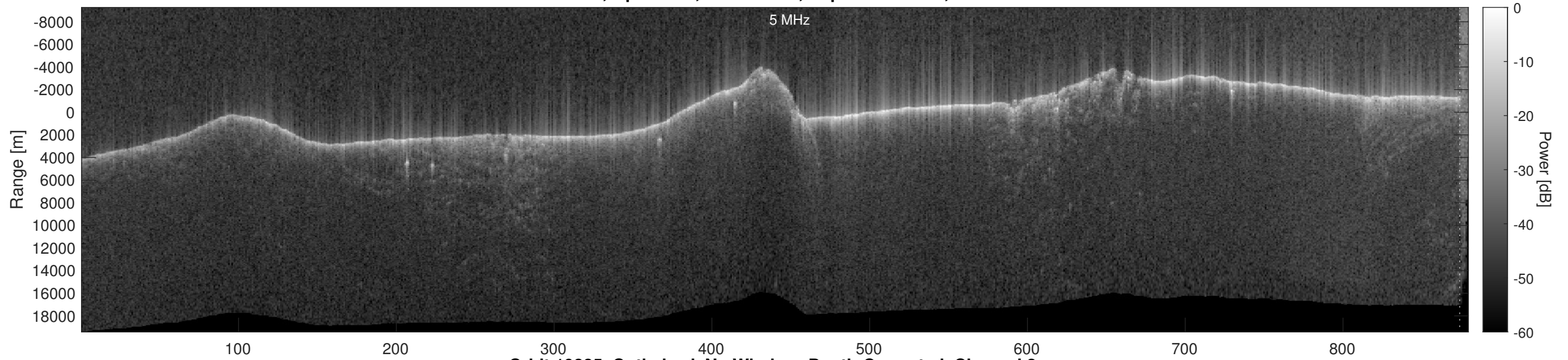
Orbit 19885, Optimized, No Window, Depth-Corrected, Channel 2
