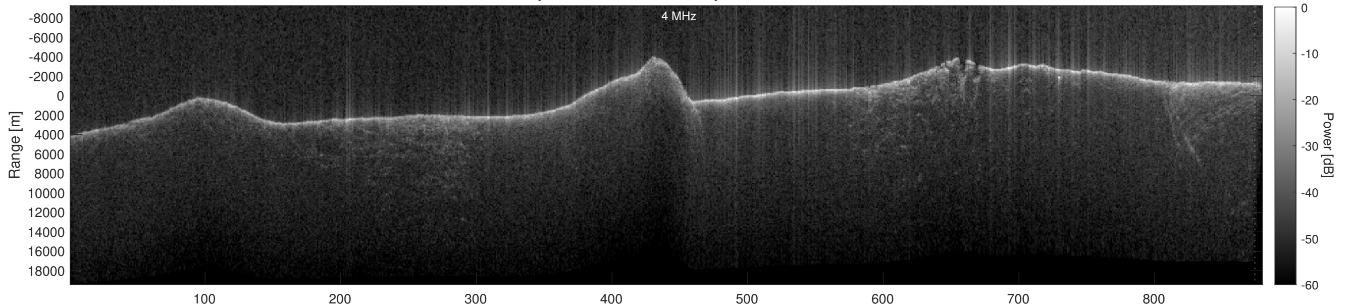
Orbit 19885, Depth-Corrected Cluttergram
