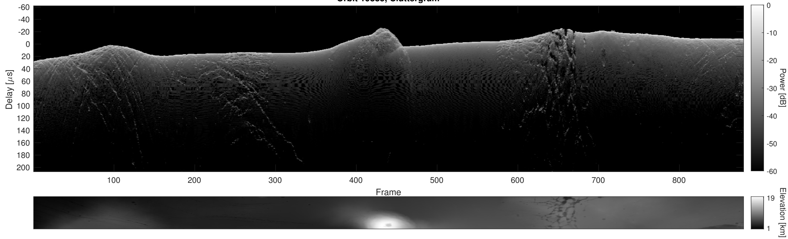
Orbit 19885, Cluttergram
