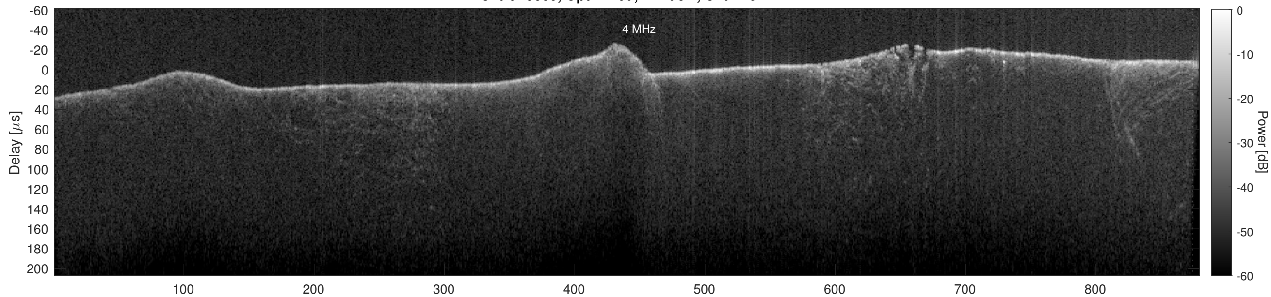
Orbit 19885, Cluttergram
