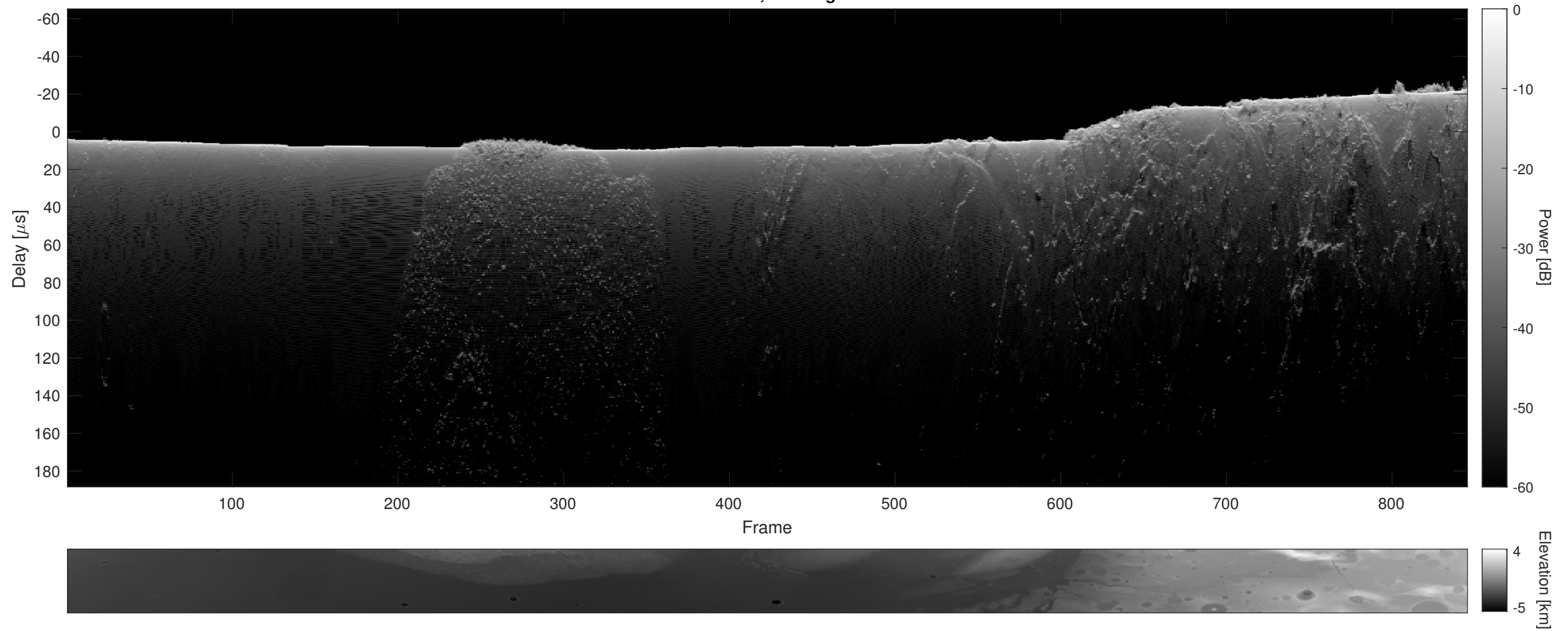
Orbit 19889, Cluttergram
