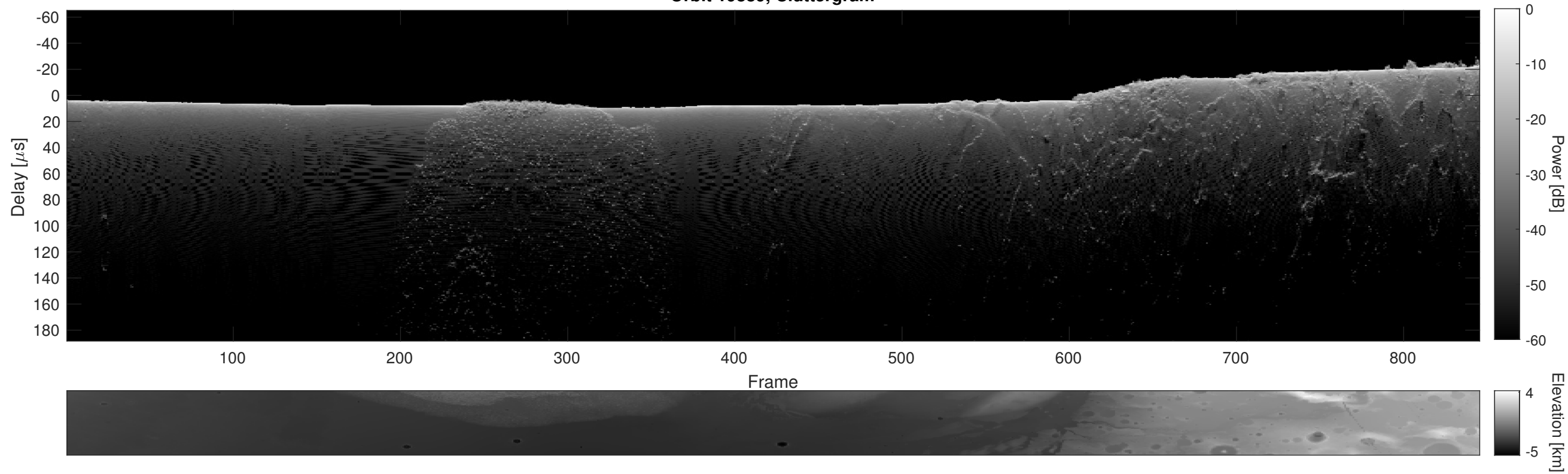
Orbit 19889, Cluttergram
