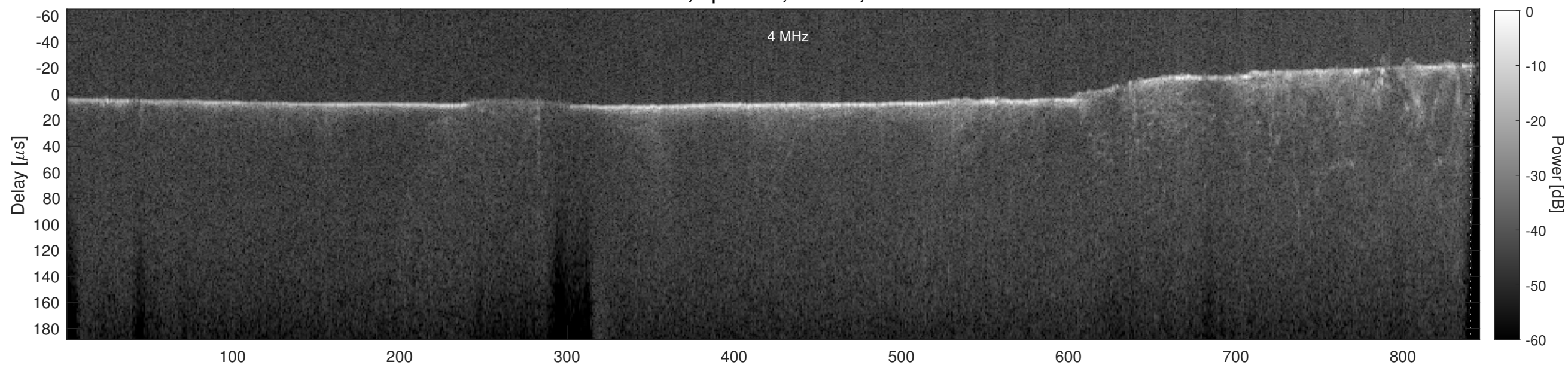
Orbit 19889, Cluttergram
