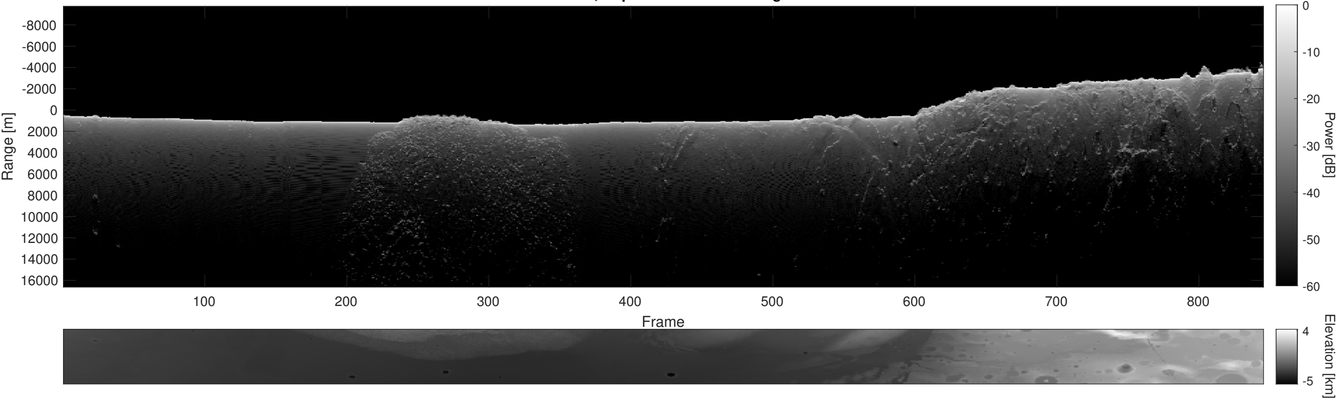
Orbit 19889, Depth-Corrected Cluttergram
