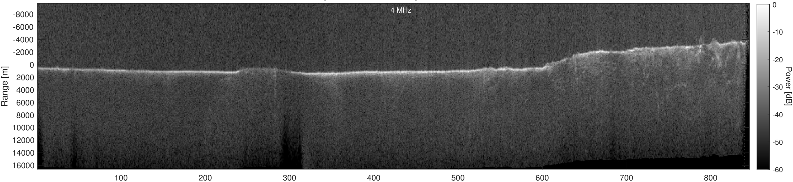
Orbit 19889, Depth-Corrected Cluttergram
