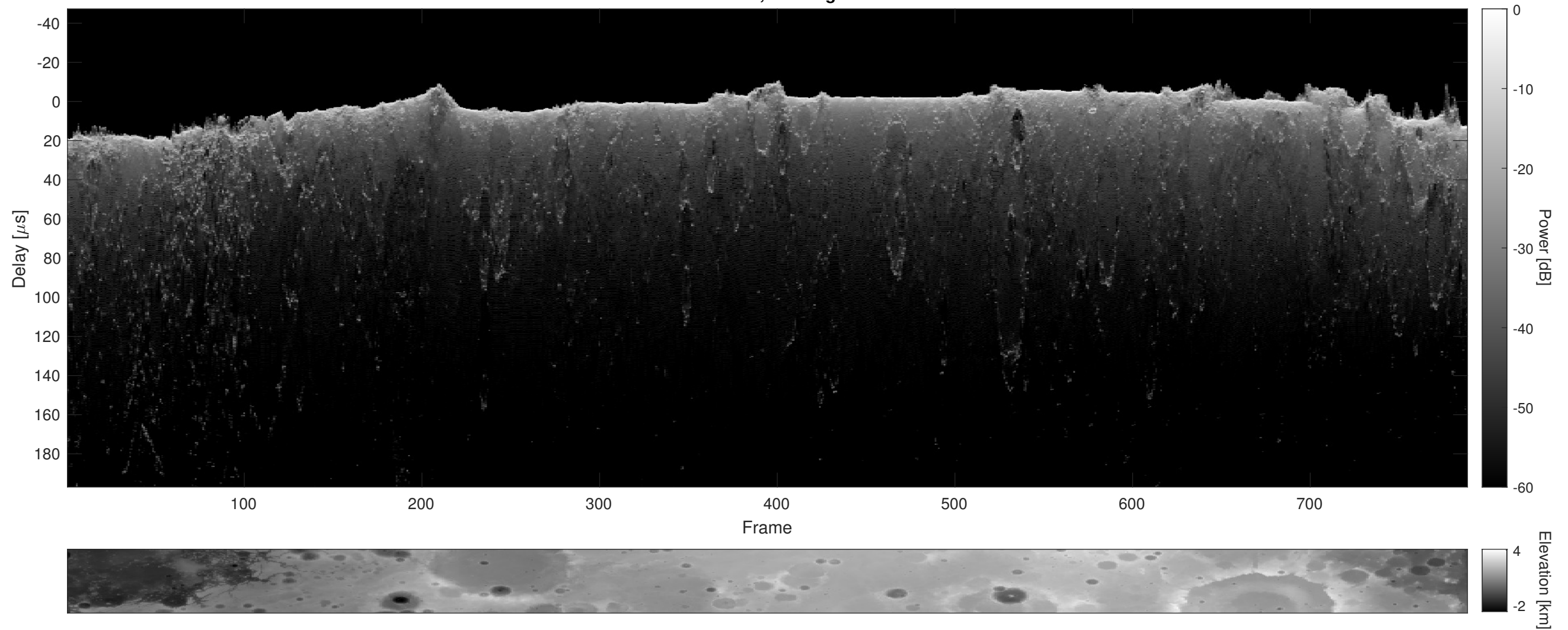
Orbit 19894, Cluttergram
